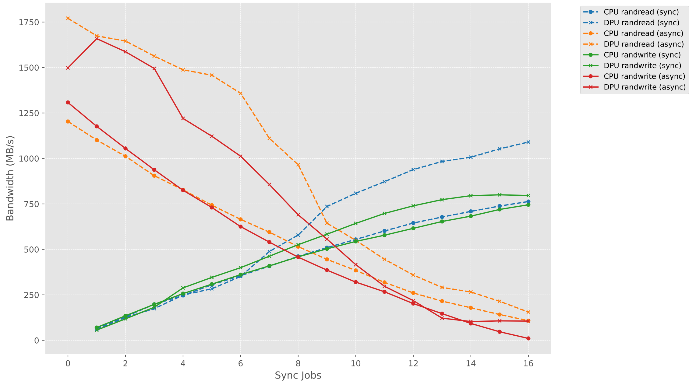
Bandwidth vs Sync Jobs (async1_syncN) - RAND (CPU vs DPU)
